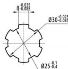
6 TEETH Ø30 RECTANGLE SPINE 6 齿矩形花键-Ø30
