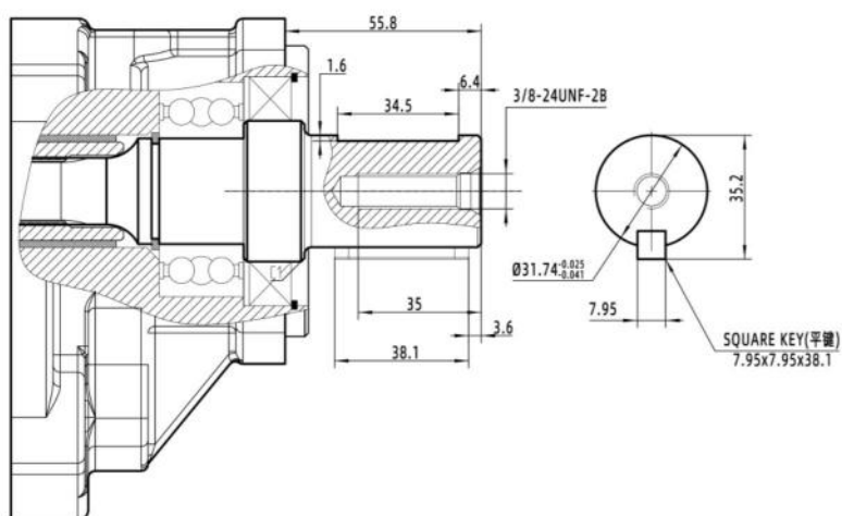
SAE 1-1/4" STRAIGHT SHAFT Φ31.75 平键
