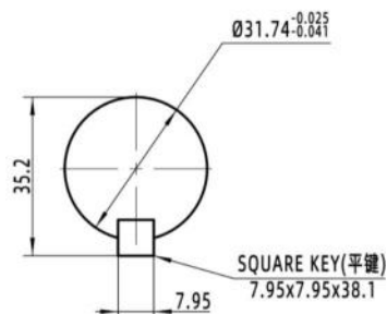
SAE-" C" 1-1/4 KEYED SHAFT \varnothing 31.75 平键
